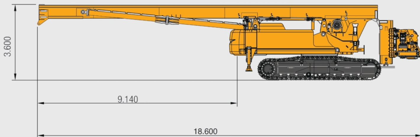
TRANSPORT POSITION
